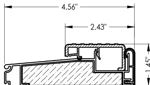
14 OUTSWING THRESHOLD
